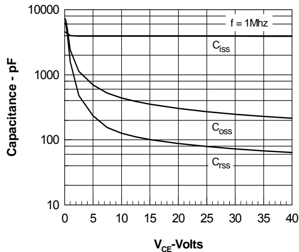
Figure 6. Capacitance Curves
