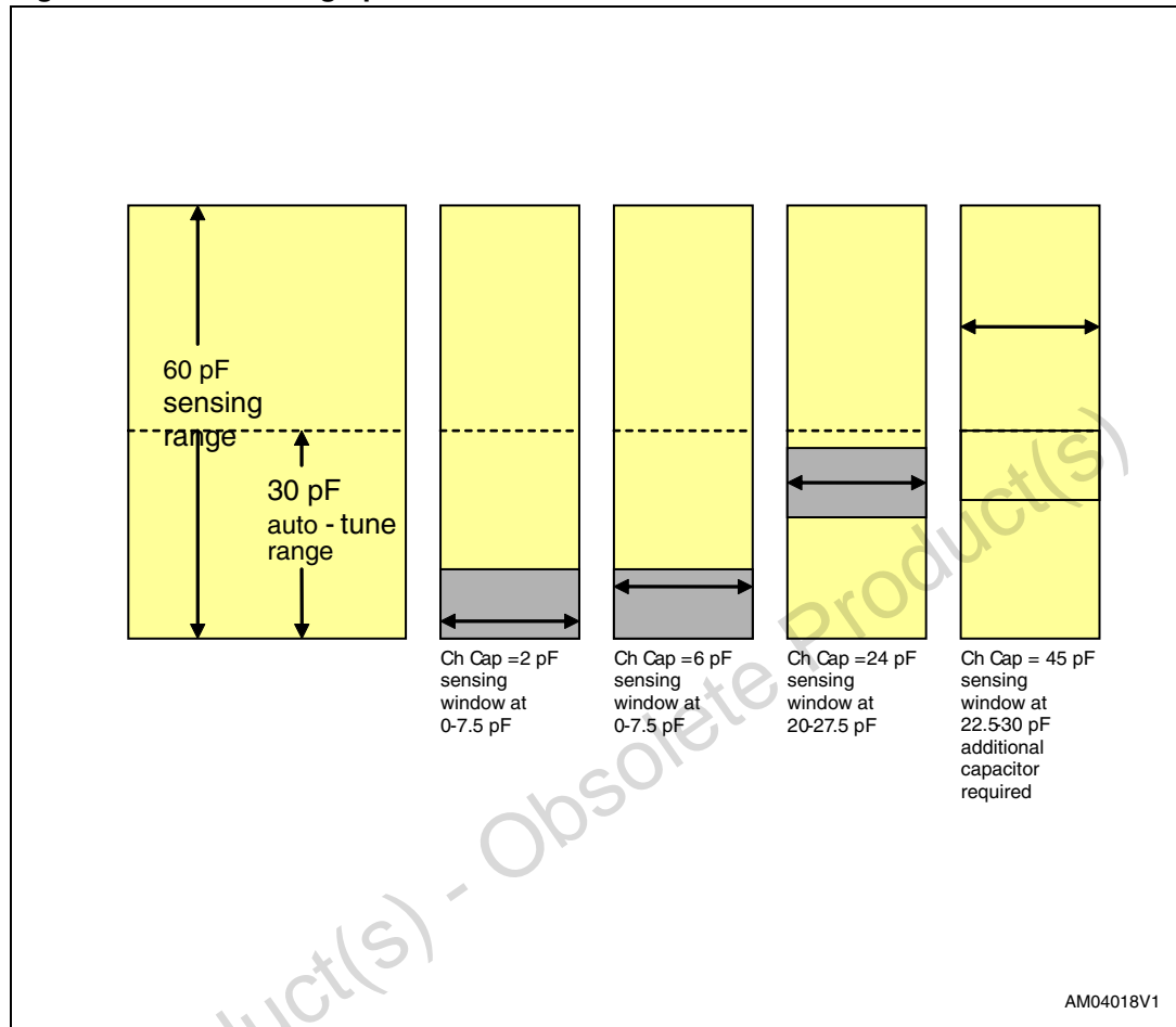
Figure 13. Auto-tuning operation
