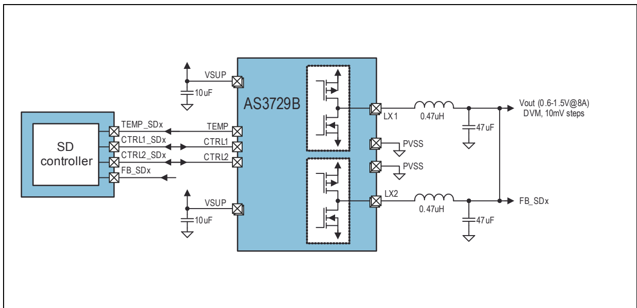
SD1 DC/DC Buck Controller: Shows basic connection of the SD1 controller to the external power stage (AS3729B) for 8A peak output current.
