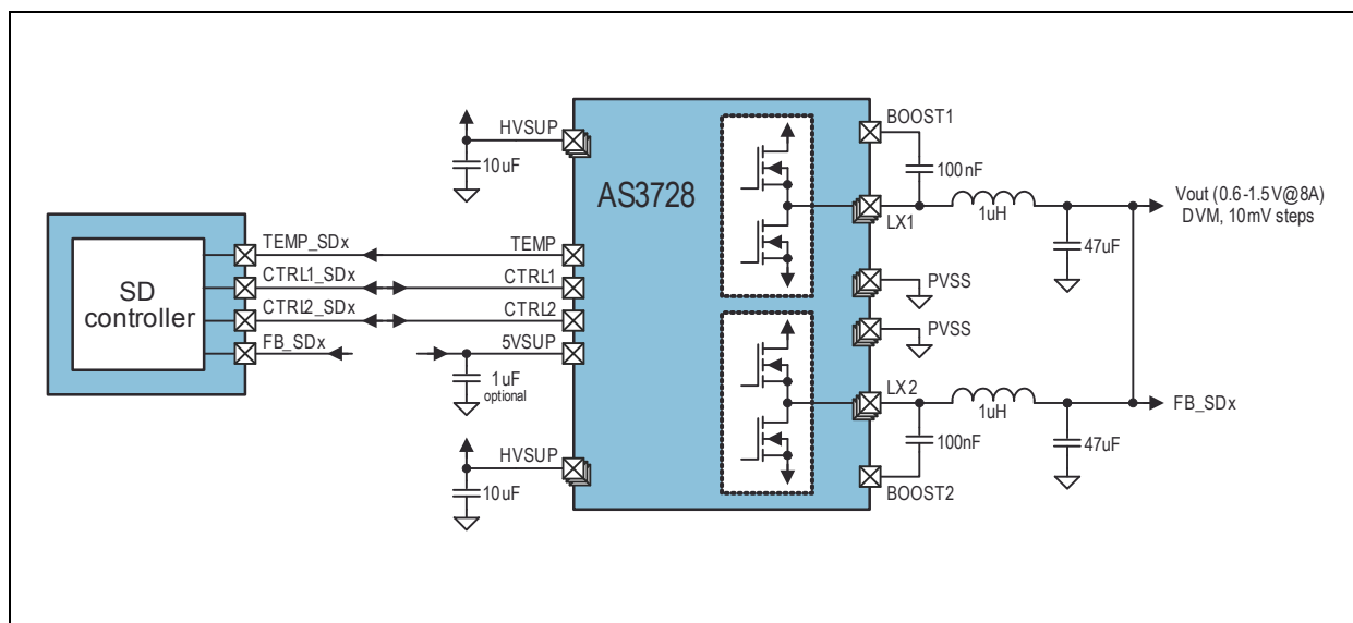
Figure 24: SD1 DC/DC Buck Controller 8A Block Diagram
