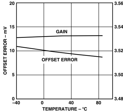
TPC 2. Offset Error and Gain vs. Temperature
