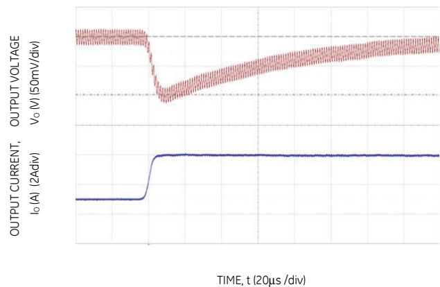
Figure 34. Transient Response to Dynamic Load Change from 50% to 100% at 12Vin, Cout = 3x47uF, CTune=1500pF & RTune=300Ω
