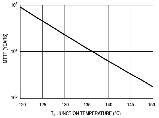
Figure 11. MTTF versus Junction Temperature NOTE: The MTTF is calculated with V_{CC} = 5 \text{ Vdc} , I_{CC} = 38 \text{ mA}
