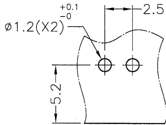
MOUNTING HOLE
