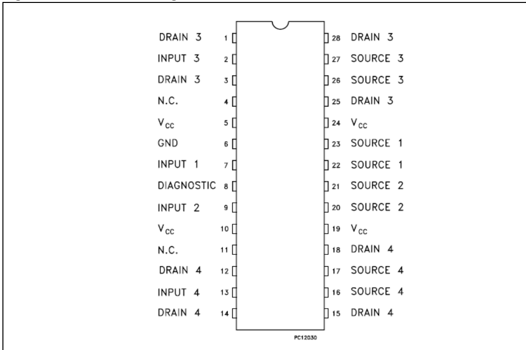
Figure 2. Connection diagram
