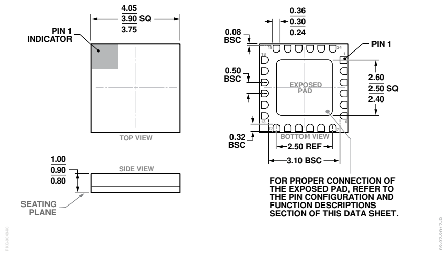
Figure 122. 24-Terminal Ceramic Leadless Chip Carrier [LCC] (E-24-1) Dimensions shown in millimeters
