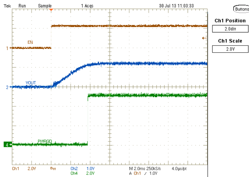
Figure 8. TPS57114EVM Startup Relative to Enable
