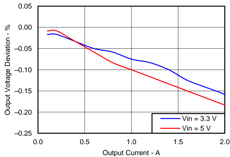
Figure 2. TPS57114EVM Load Regulation
