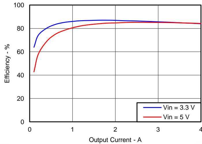
Figure 1. TPS57114EVM Efficiency
