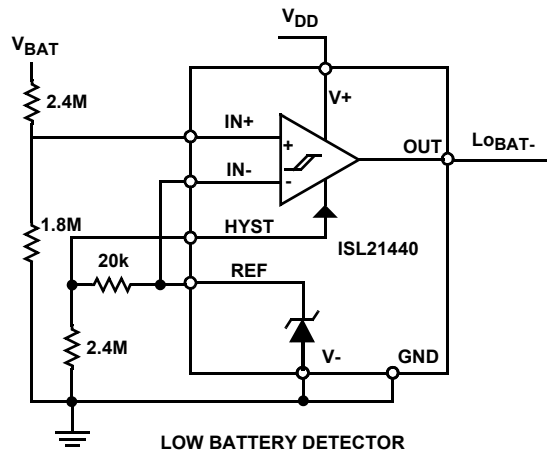
FIGURE 1. TYPICAL APPLICATION
