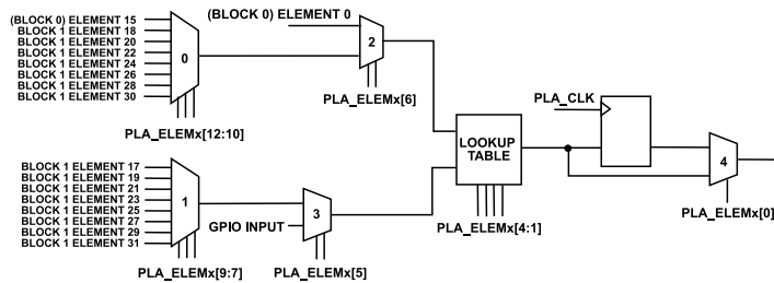
Figure 31. PLA Element: Block 0, Element 1 to Element 15
