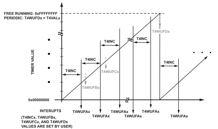
Figure 27. Wake-Up Timer Fields Action
