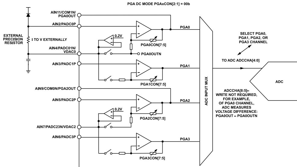
Figure 6. PGA Amplifier in DC PGA Gain Mode
