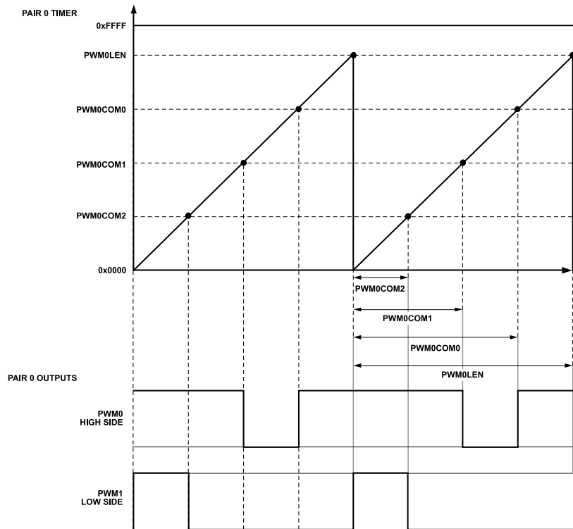
Figure 36. Waveform of PWM Channel Pair in Standard Mode
