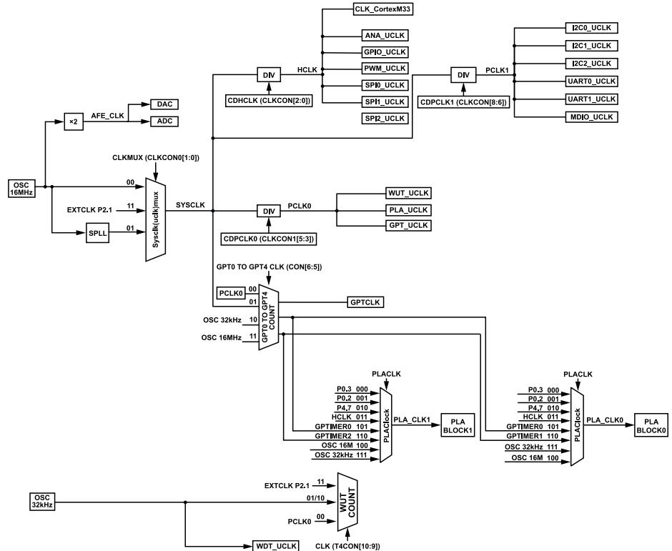
Figure 1. Clock Architecture Overview
