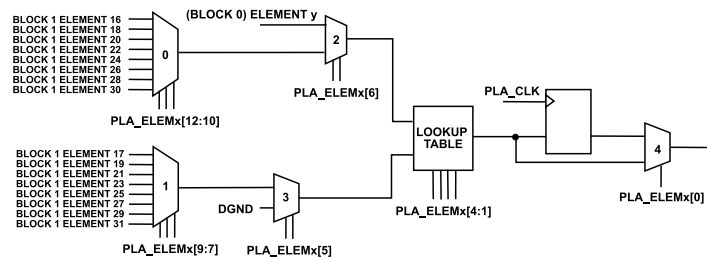
Figure 32. PLA Element: Block 1, Element 16
