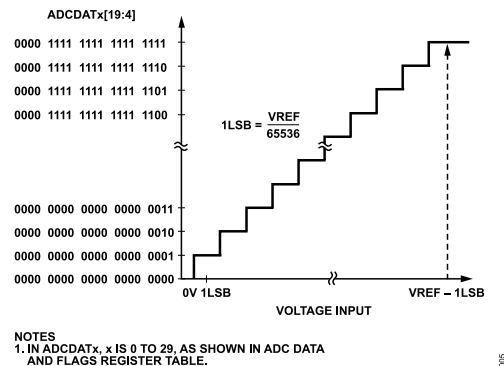
Figure 4. ADC Transfer Function: Single-Ended Mode
