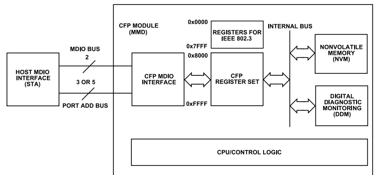
Figure 23. CFP Management interface Architecture
