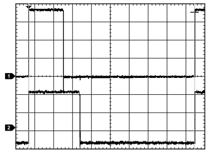
Figure 37. PWM Output on PWM0 and PWM1 (PWM Channel 2)
