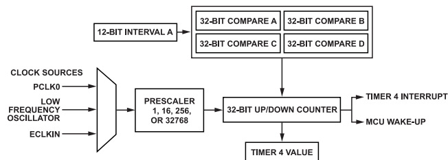
Figure 26. Wake-Up Timer Block Diagram
