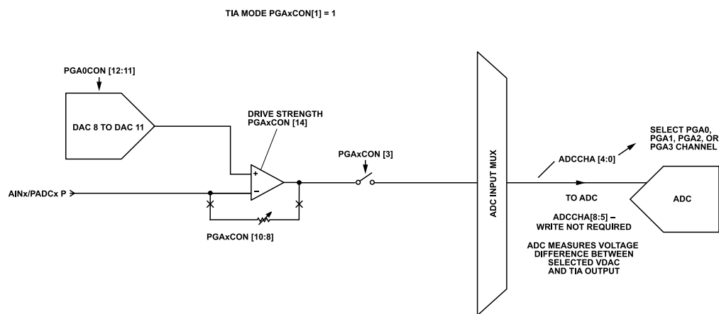
Figure 5. PGA Amplifier in TIA Mode
