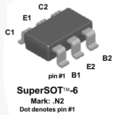
Figure 1. Device Package
