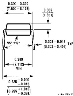
Molded Dual-In-Line Pkg. (N) Order Number LMC660AIN, LMC660CN or LMC660EN NS Package Number N14A
