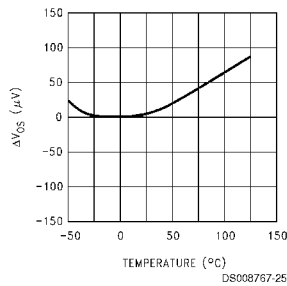
Offset Voltage
