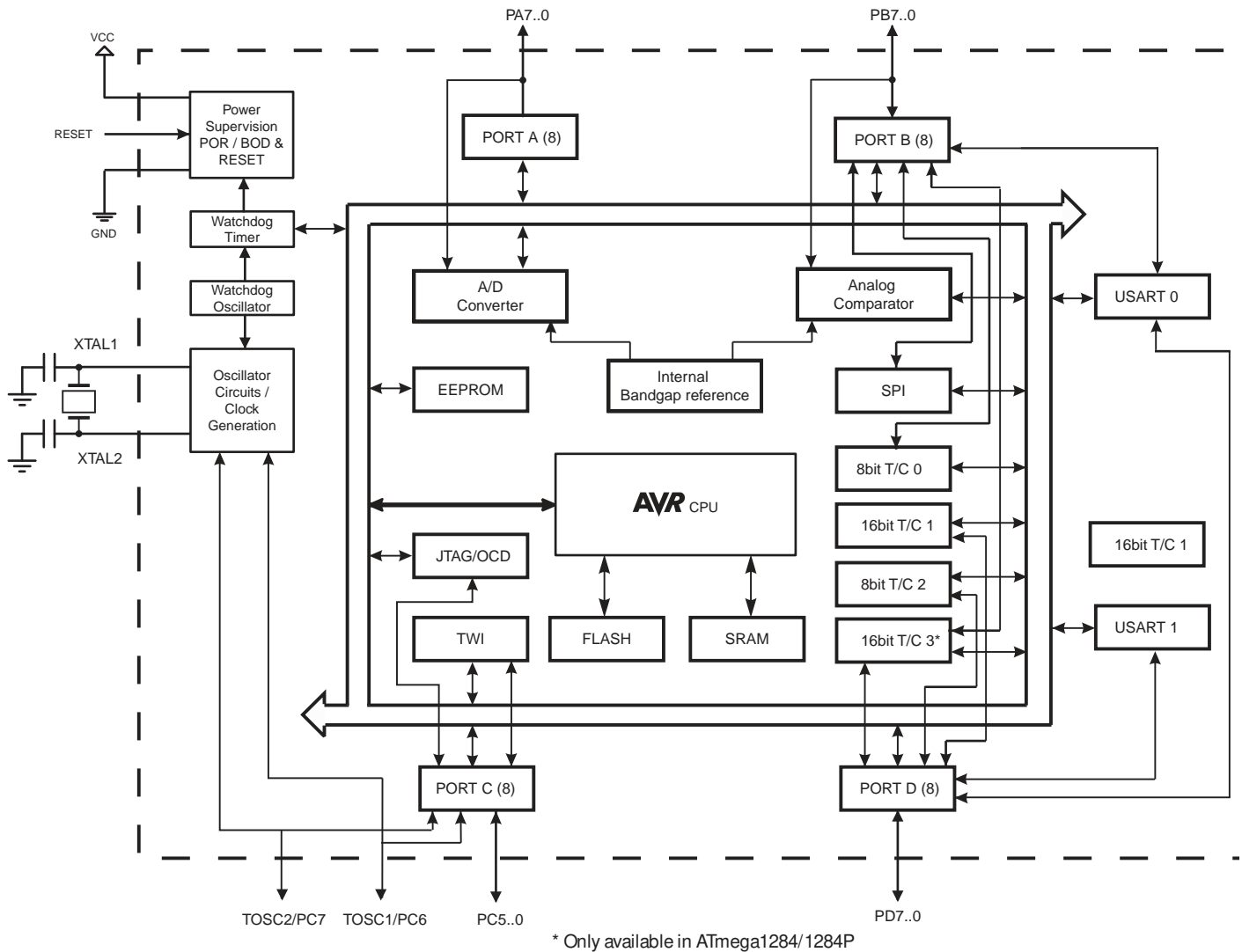
Figure 2-1. Block diagram
