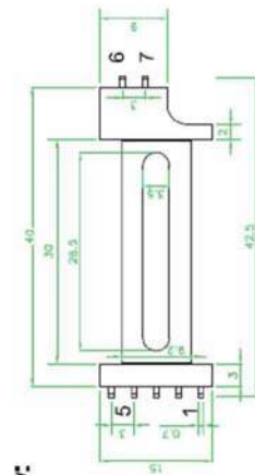
Bottom View: Unit: mm
