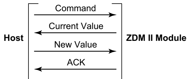
Figure 6. Write Command Structure
