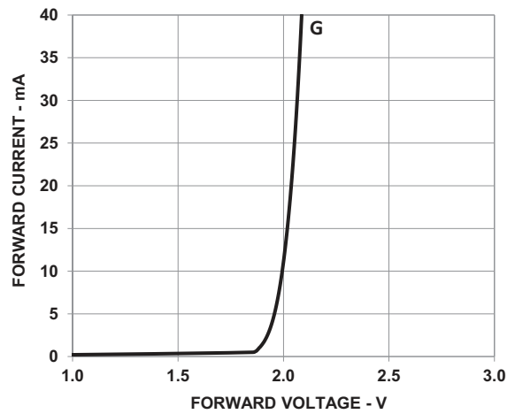
Figure 4: Forward Current vs. Forward Voltage
