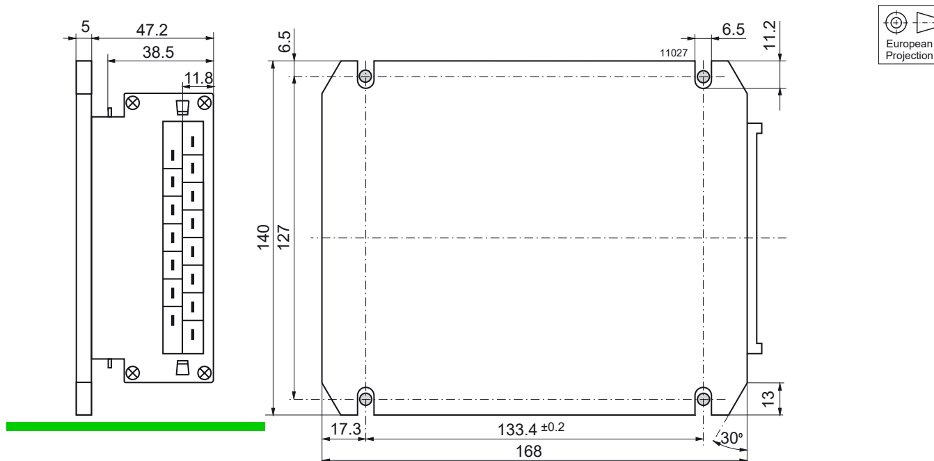
Fig. 15 Option B, large cooling plate Weight: 1.3 kg
