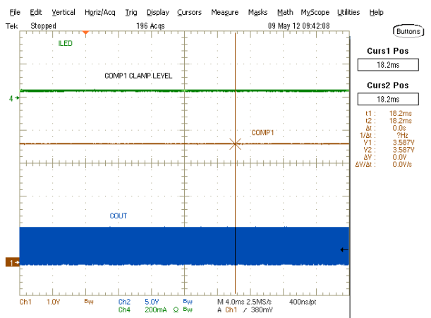
Figure 26 · COMP1 Clamp Level
