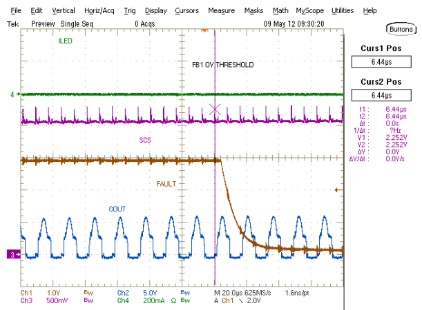
Figure 24 · FB1 OV Threshold
