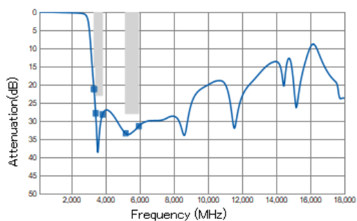
Attenuation (Low-Band)
