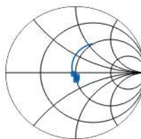
Smith Chart (Low-Band)
