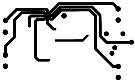
Recommended SOP PC Board Layout: Bottom Layer
