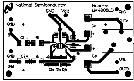
Recommended LD PC Board Layout: Top Layer
