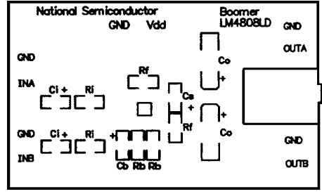
Recommended LD PC Board Layout: Top Silkscreen
