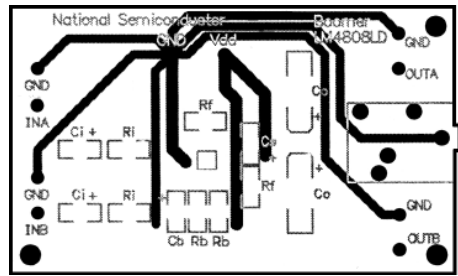
Recommended LD PC Board Layout: Bottom Layer
