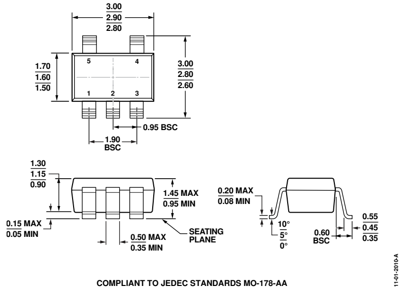
COMPLIANT TO JEDEC STANDARDS MO-178-AA Figure 66. 5-Lead Small Outline Transistor Package [SOT-23] (RJ-5) Dimensions shown in millimeters
