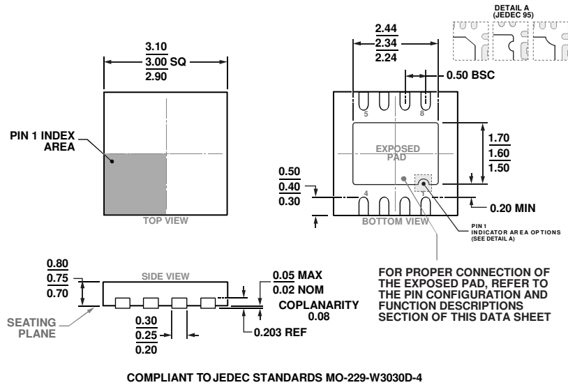
COMPLIANT TO JEDEC STANDARDS MO-229-W3030D-4 Figure 67. 8-Lead Lead Frame Chip Scale Package [LFCSP] 3 mm x 3 mm Body and 0.75 mm Package Height (CP-8-11) Dimensions shown in millimeters
