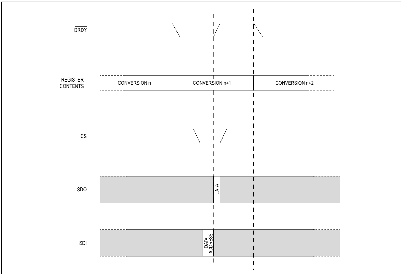
Figure 7. DRDY Operation
