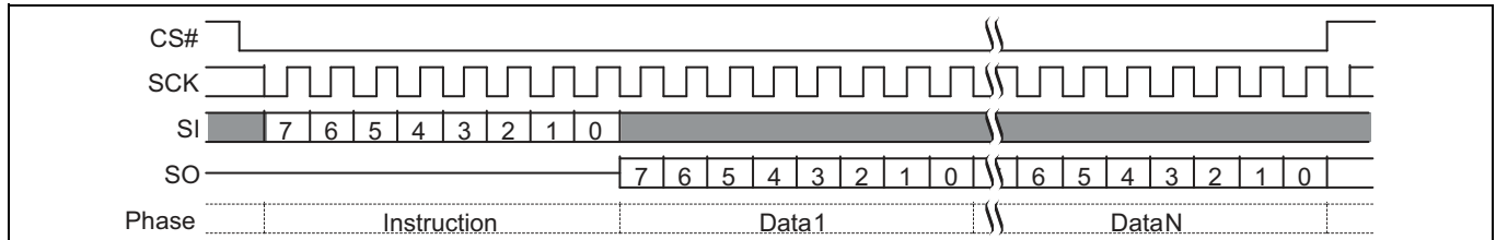
Figure 50 Read Identification (RDID) command sequence
