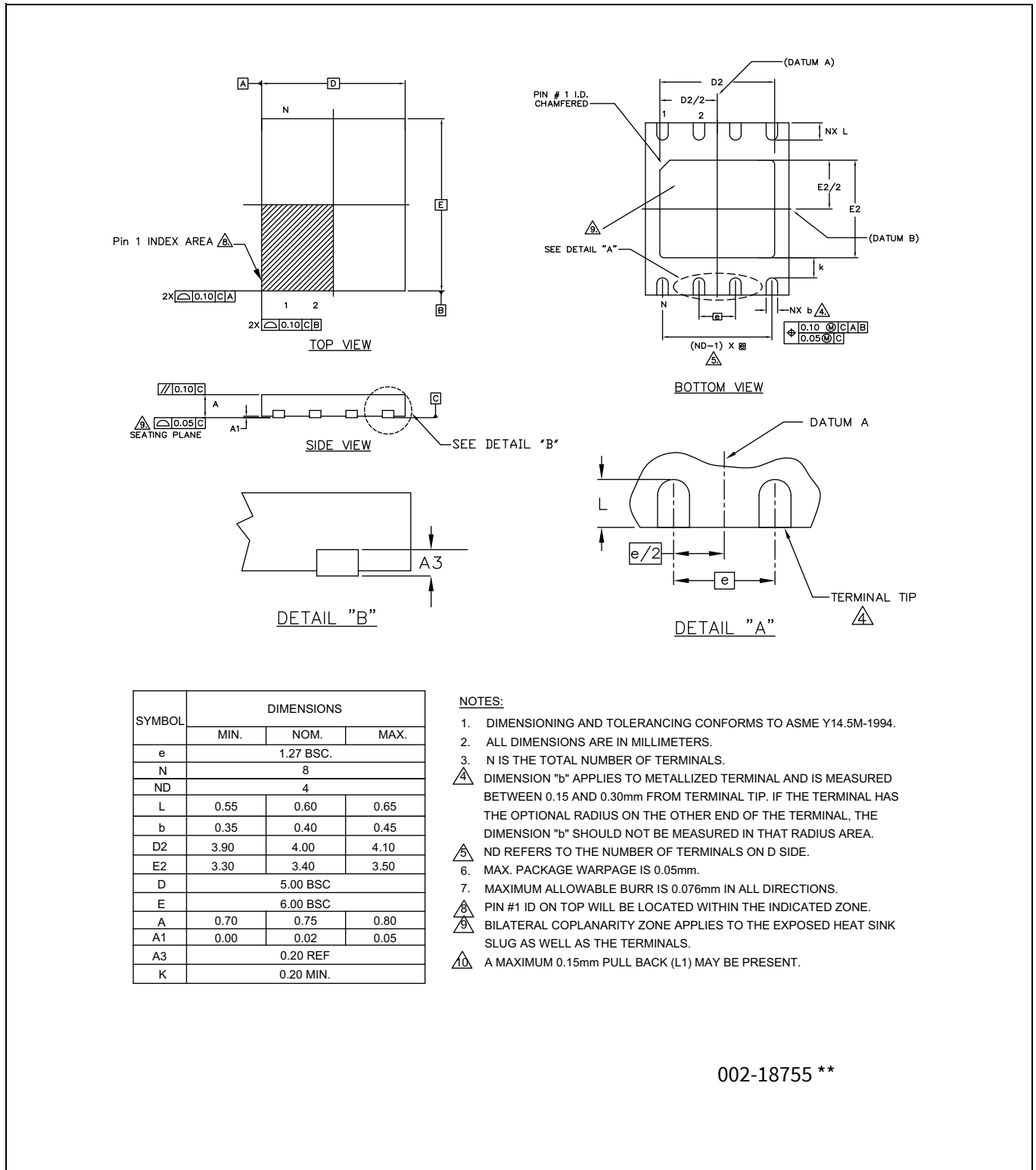
Figure 41 8-lead DFN ((5.0 x 6.0 x 0.8 mm) 4.0 x 3.4 mm E-pad (sawn)) package outline, 002-18755
