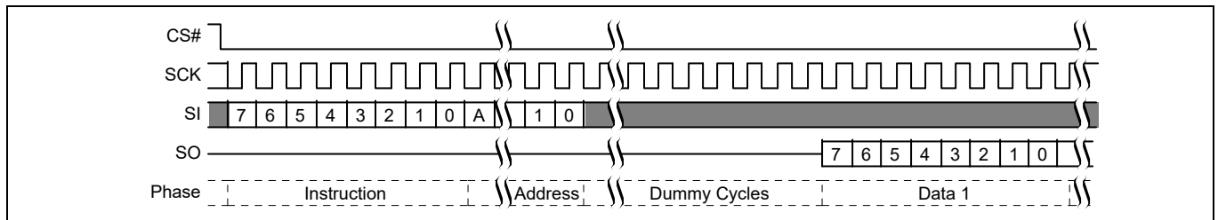
Figure 68 ECC Status Register Read command sequence [49, 50]
