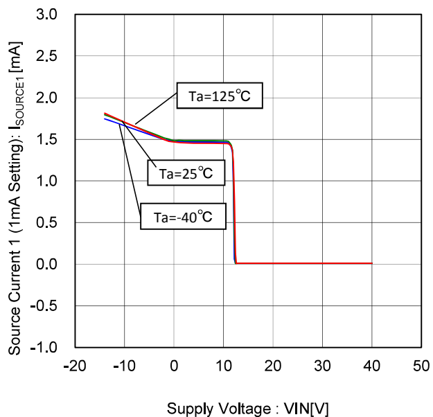
Figure 34. Source Current 1- Voltage Characteristic (1mA Setting)
