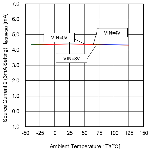
Figure 41. Source Current 2- Temperature Characteristic (3mA Setting)
