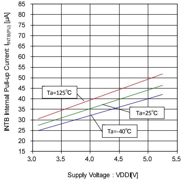
Figure 100. INTB Internal Pull-up Current- Voltage Characteristic
