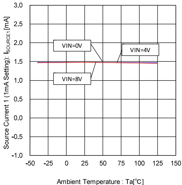
Figure 33. Source Current 1- Temperature Characteristic (1mA Setting)
