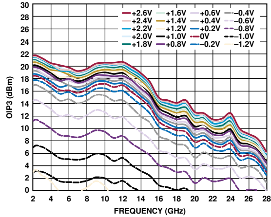
Figure 35. OIP3 vs. Frequency at Various V_{GG2} Voltages
