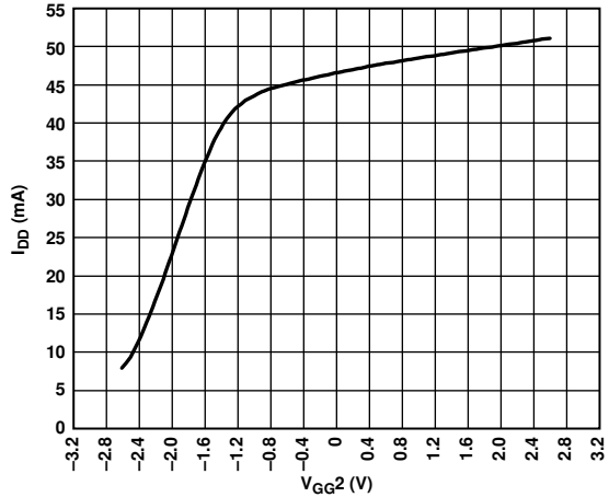
Figure 36. I_{DD} vs. V_{GG2} Voltages, V_{DD} = 5V
