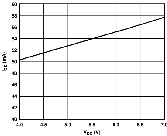
Figure 34. I_{DD} vs. V_{DD}
