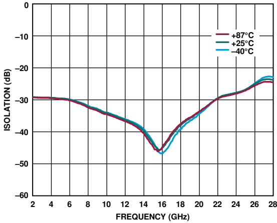
Figure 33. Isolation vs. Frequency over Various Temperatures
