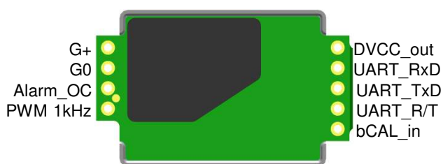
Figure 2. Pin assignment
