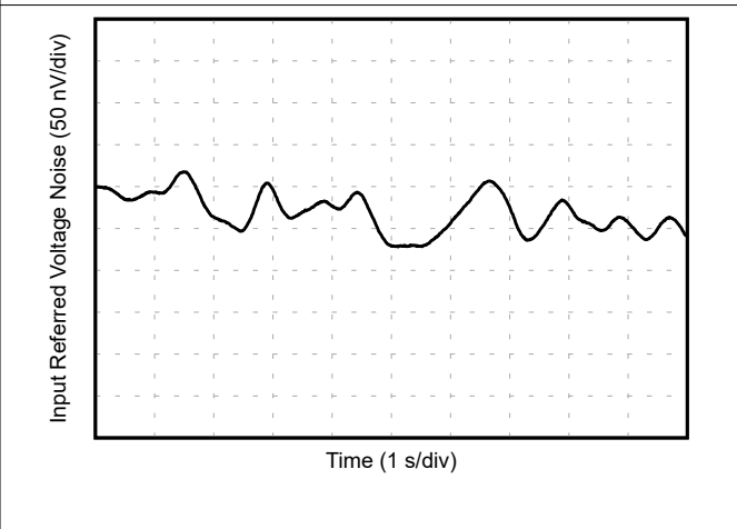
Figure 6-24. 0.1-Hz To 10-Hz Noise
