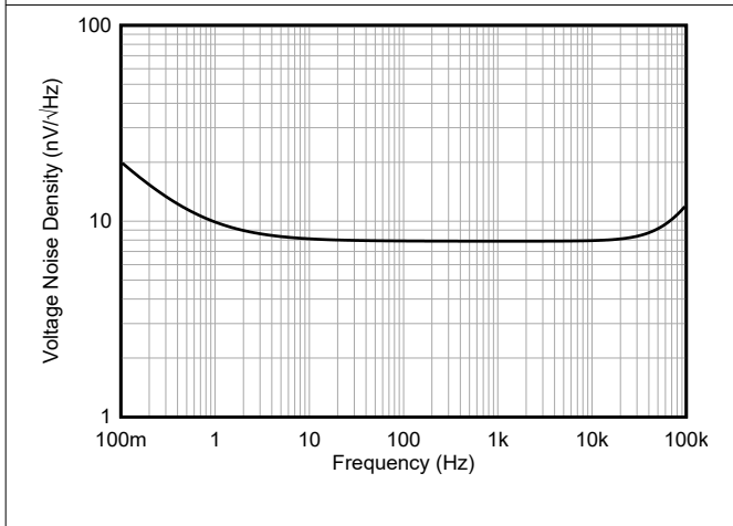
Figure 6-23. Voltage Noise Density vs Frequency
