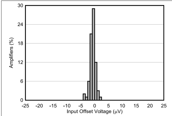
Figure 6-1. Offset Voltage Production Distribution at 25°C
