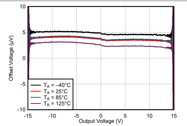
Figure 6-6. Offset Voltage vs Output Voltage
