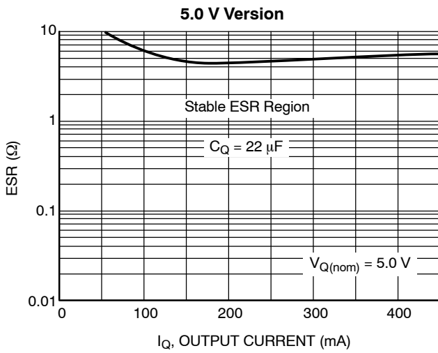
Figure 2. Output Stability with Output Capacitor ESR
