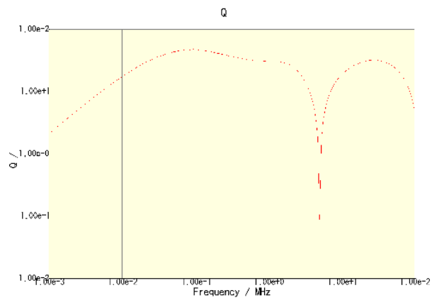
CLF6045T-680M-CA
