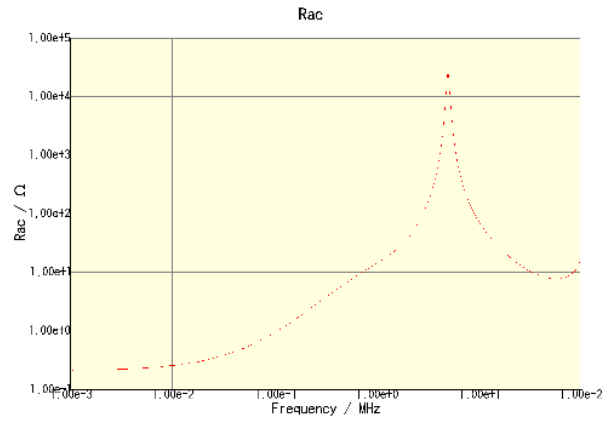
CLF6045T-680M-CA
