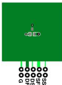
a) 80\text{ }^\circ\text{C}/\text{W} when mounted on a 1\text{ in}^2 pad of 2 oz copper
