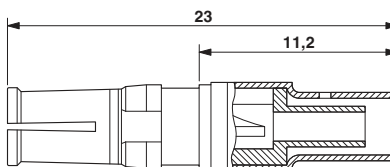
Dimensioned drawing
