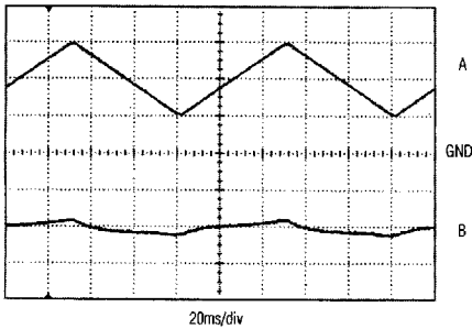
STEP-UP/STEP-DOWN OPERATION
