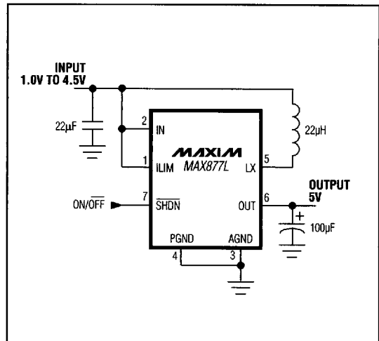
Figure 4. MAX877L Standard Application Circuit
