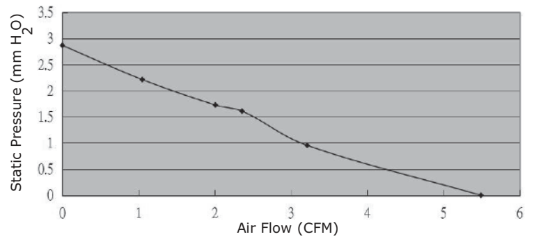
CFM-4010C-265-251
