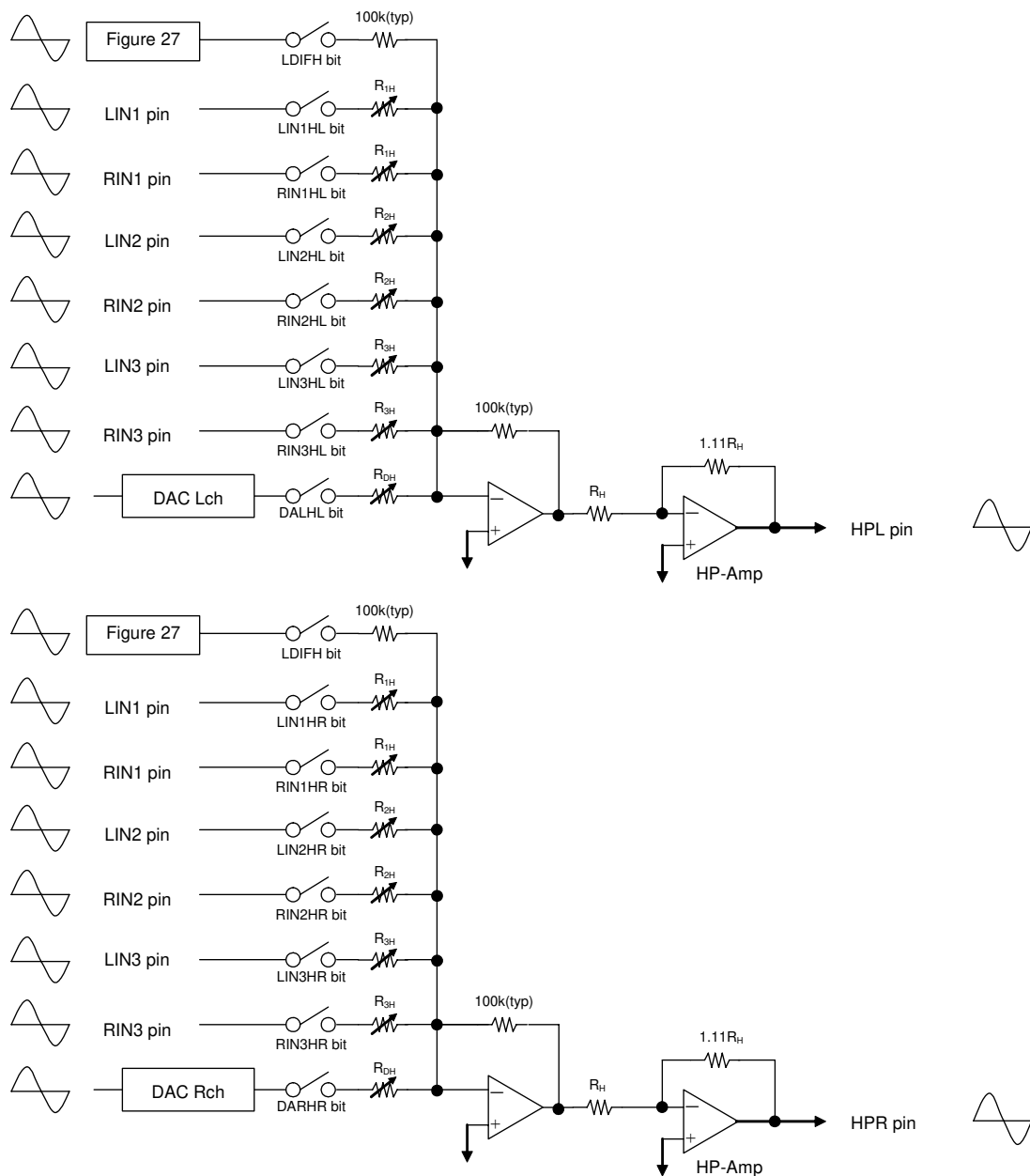
Figure 25. Summation circuit for HPL/R output
