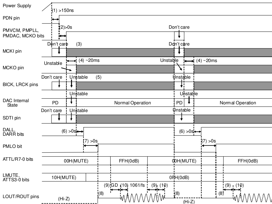
Figure 36. Power-up/down sequence of DAC and LO/RO (Don't care: except Hi-Z)
