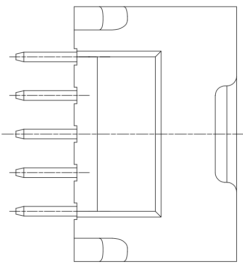
ENGAGEMENT FIGURE (2:1)
