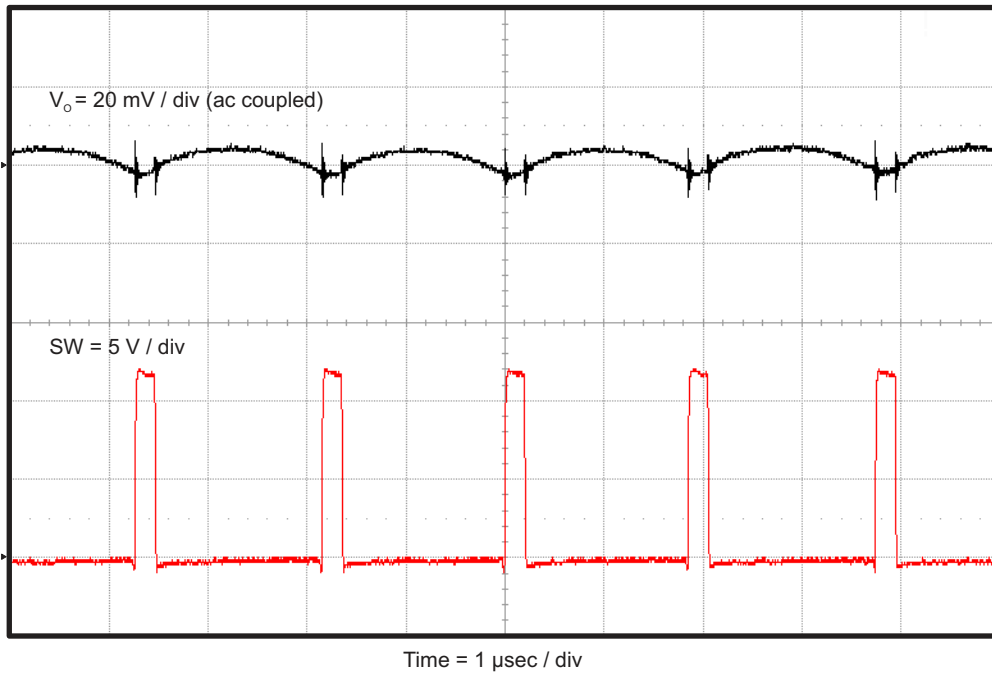
Figure 4-7. TPS562210EVM-663 Output Voltage Ripple, I_{OUT} = 2 \text{ A}
