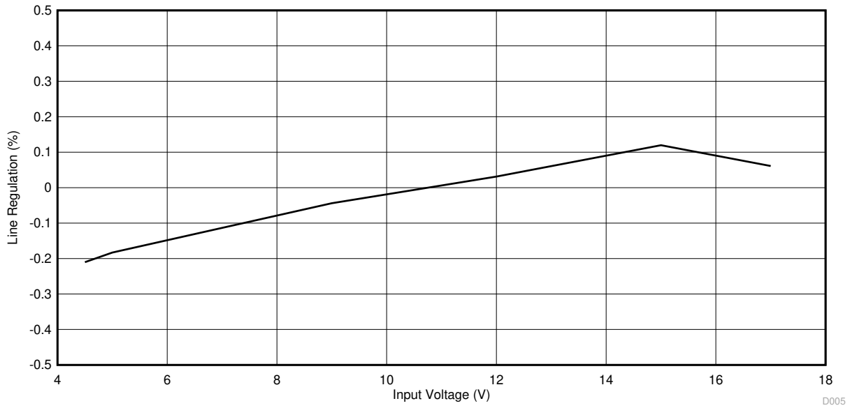
Figure 4-5. TPS562210EVM-663 Line Regulation
