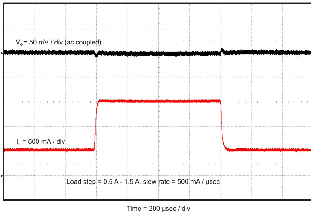
Figure 4-6. TPS562210EVM-663 Load Transient Response, 25% to 75% Load Step
