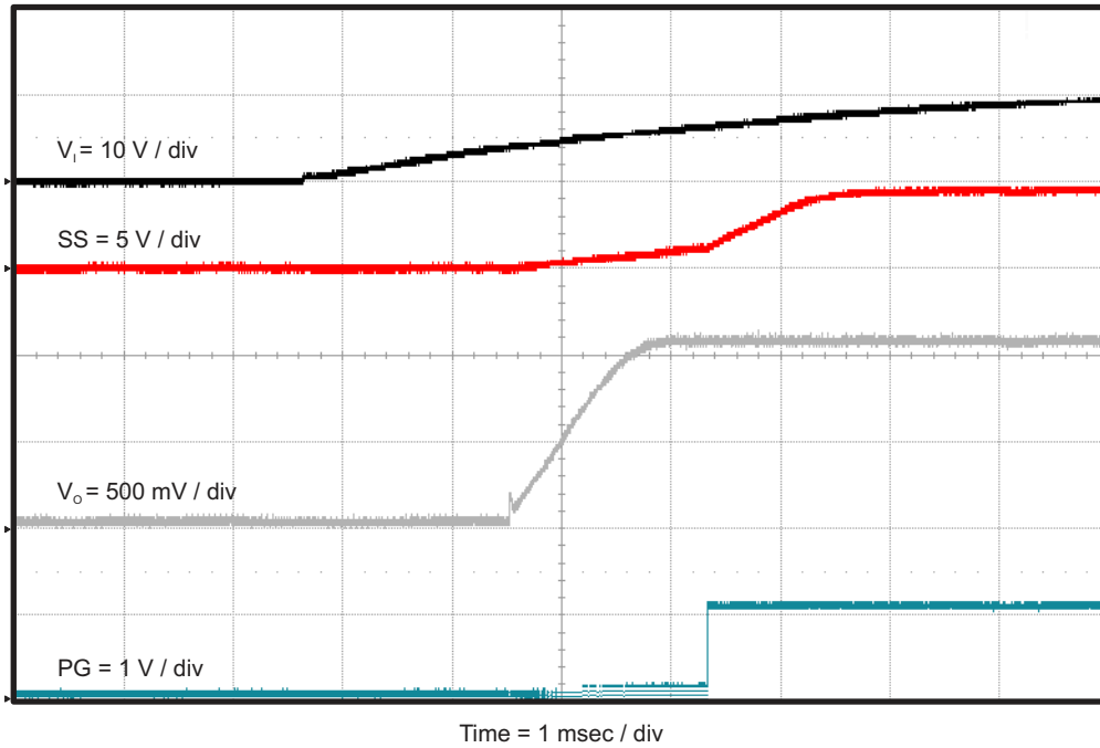
Figure 4-11. TPS562210EVM-663 Start-Up Relative to V_{IN}
