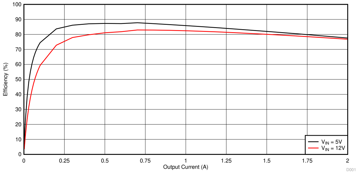
Figure 4-1. TPS562210EVM-663 Efficiency
