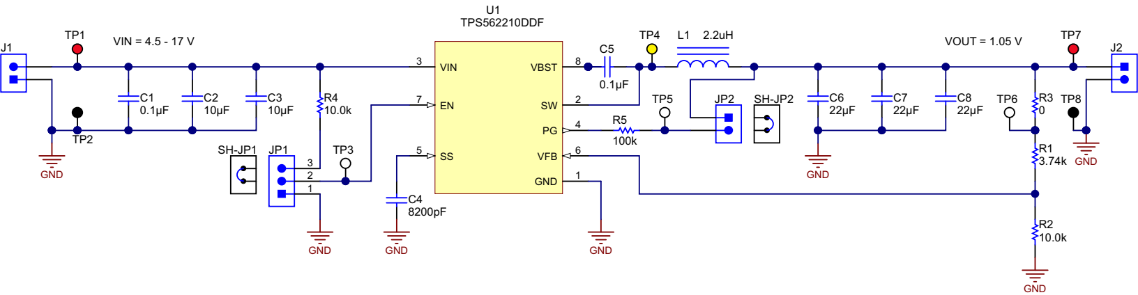
Figure 6-1. TPS562210EVM-663 Schematic Diagram
