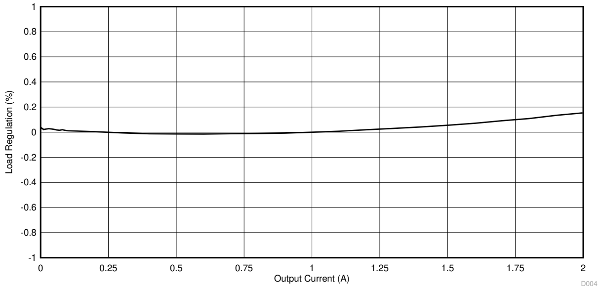
Figure 4-4. TPS562210EVM-663 Load Regulation, 12 V Input
