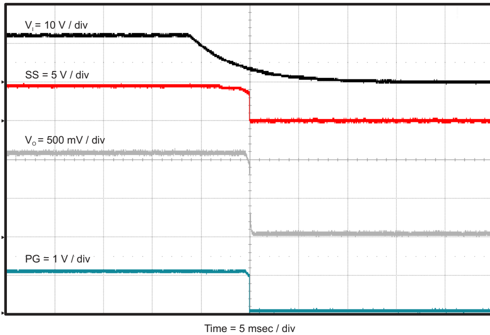
Figure 4-13. TPS562210EVM-663 Shut-Down Relative to V_{IN}
