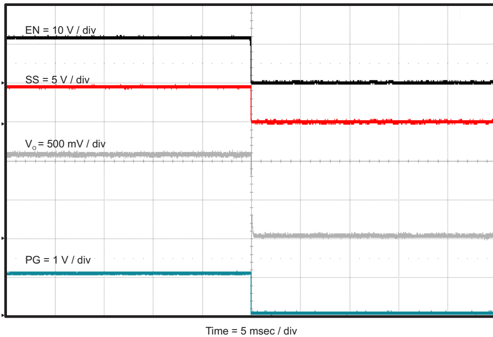
Figure 4-14. TPS562210EVM-663 Shut-Down Relative to EN
