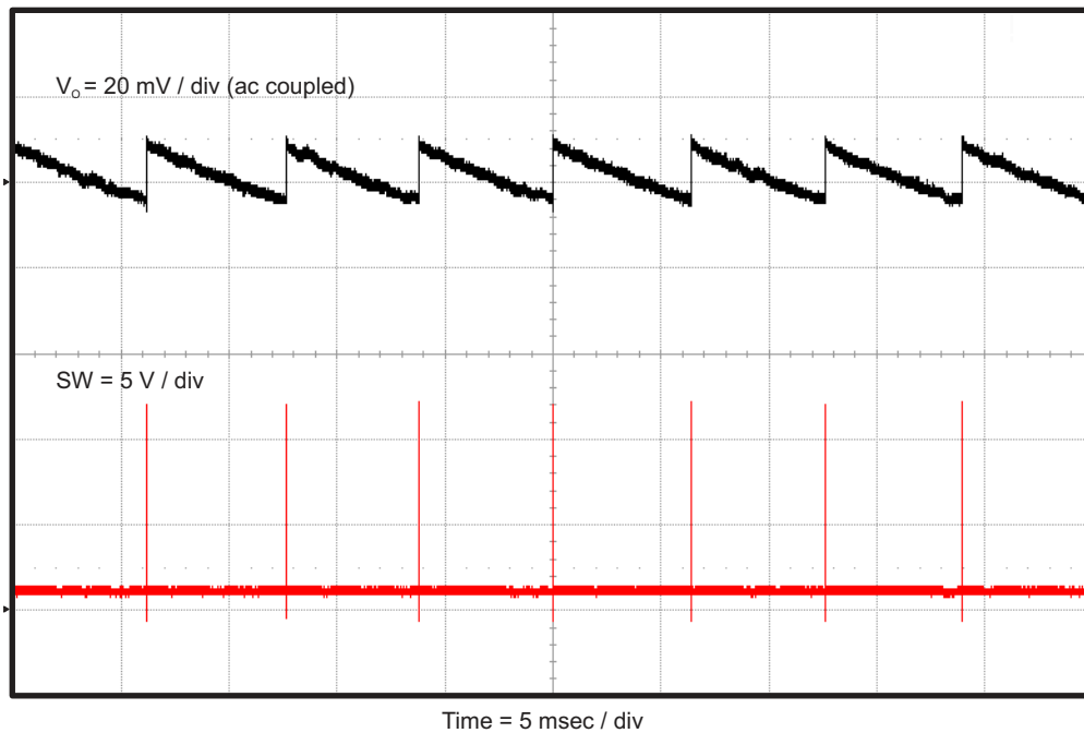
Figure 4-9. TPS562210EVM-663 Output Voltage Ripple, I_{OUT} = 0 \text{ mA}
