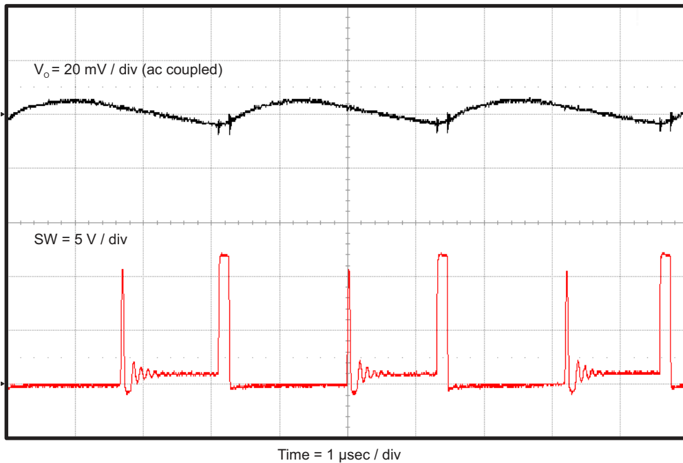
Figure 4-8. TPS562210EVM-663 Output Voltage Ripple, I_{OUT} = 200 \text{ mA}
