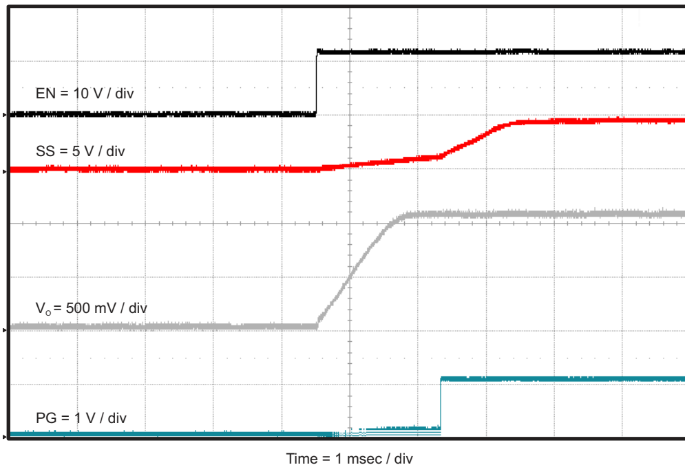
Figure 4-12. TPS562210EVM-663 Start-Up Relative to EN
