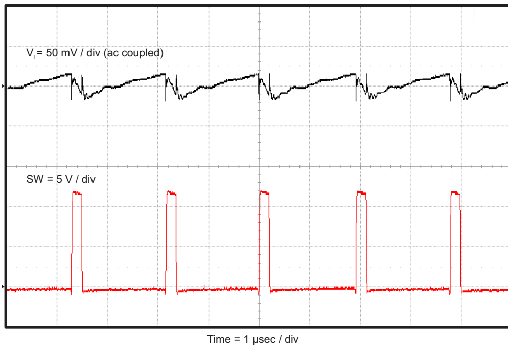
Figure 4-10. TPS562210EVM-663 Input Voltage Ripple, I_{OUT} = 2 \text{ A}
