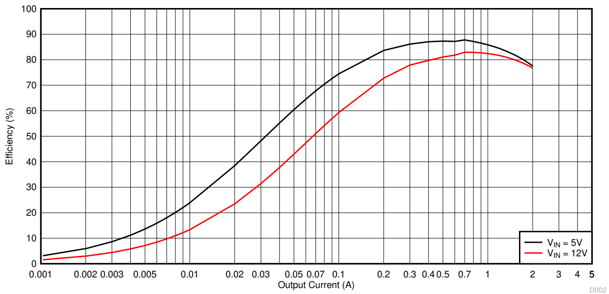
Figure 4-2. TPS562210EVM-663 Light Load Efficiency
