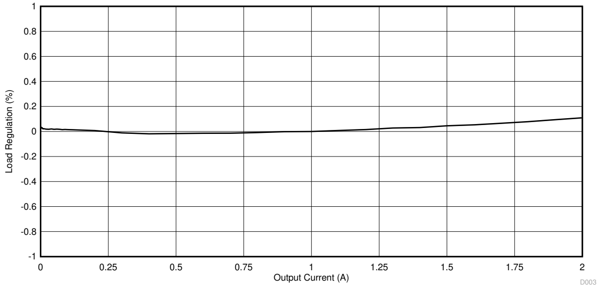
Figure 4-3. TPS562210EVM-663 Load Regulation, 5 V Input
