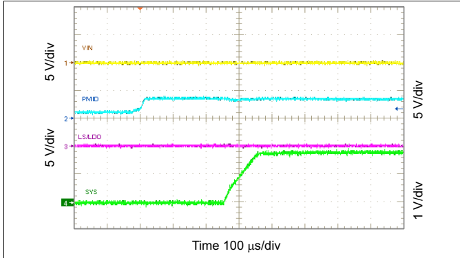
Figure 36. Battery Connected to V (BAT)
