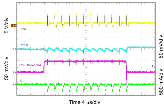
Figure 67. 1.2 V VSYS Load Transient, 0 to 50 mA
