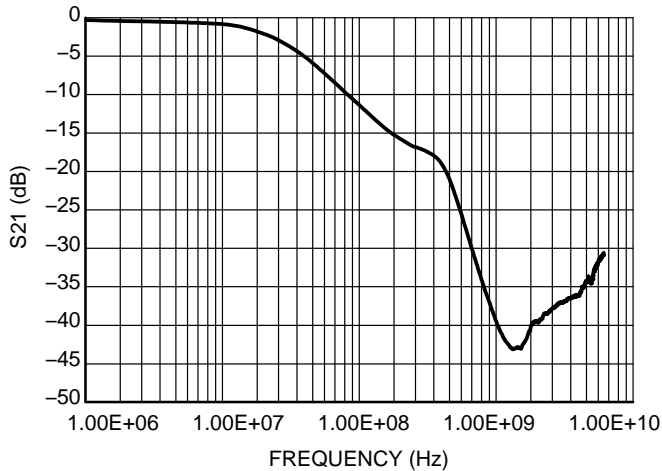
Figure 1. Typical Insertion Loss Characteristics (S21 Measurement)
