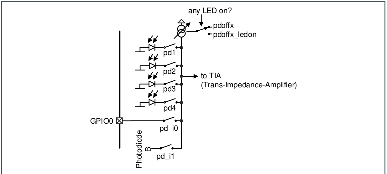
Figure 21: Photodiode Selection
