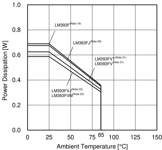
(c) LM393xxx
