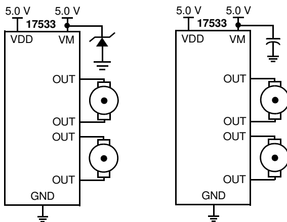
Figure 7. CEMF Snubbing Techniques
