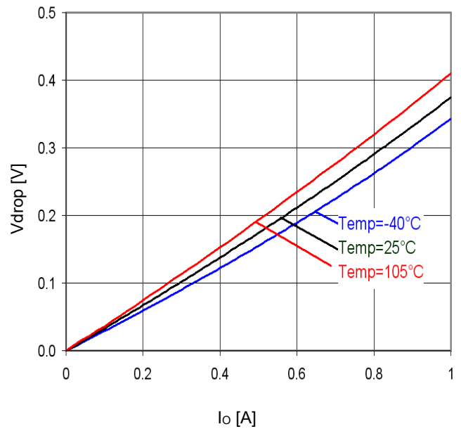
Fig.34 Minimum dropout Voltage 2 (Vcc=2.4V, Ta=25°C)
