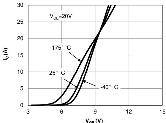
Figure 3: Transfer Characteristic
