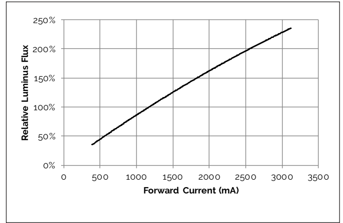
Figure 11: V18C Typical Relative Flux vs. Current ( T_c = 25^\circ\text{C} )
