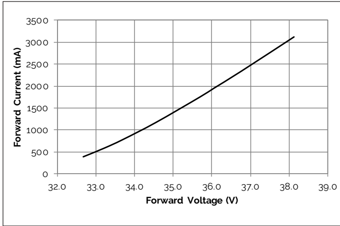
Figure 10: V18C Drive Current vs. Voltage ( T_c = 25^\circ\text{C} )
