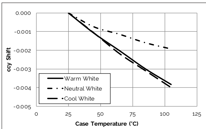
Figure 14: Typical ccy Shift vs. Case Temperature
