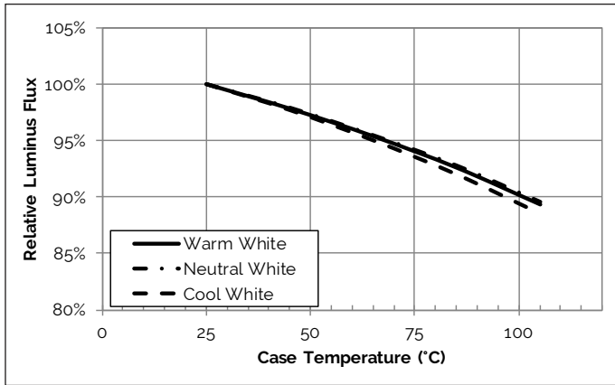
Figure 12: Typical DC Flux vs. Case Temperature
