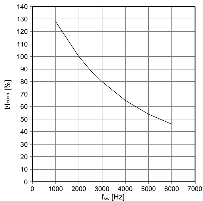
fsw - derating curve IGBT (motor) cos(phi) = 0,85 T cool medium = 40°C
