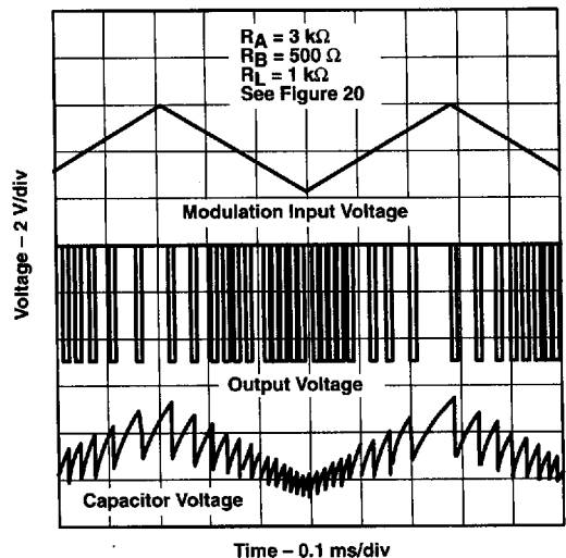
Figure 21. Pulse-Position-Modulation Waveforms
