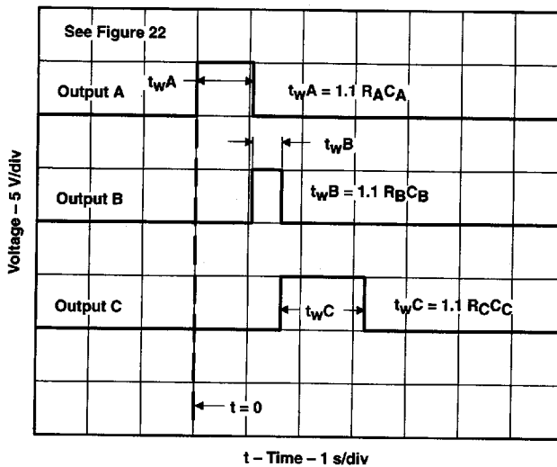
Figure 23. Sequential Timer Waveforms
