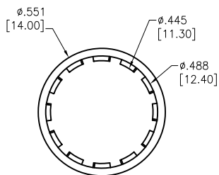
WASHER
