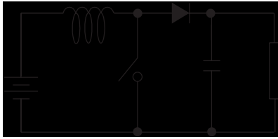
Figure 3. Basic Boost Circuit
