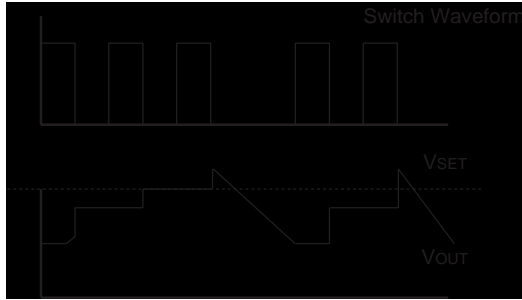
Figure 5. PFM Waveform
